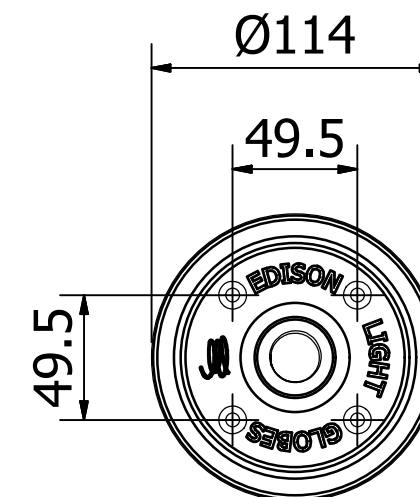
CEILING PLATE MOUNTING DETAIL
