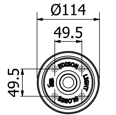
CEILING PLATE MOUNTING DETAIL
